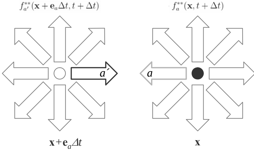
Figure 78. Probabilistic bounceback. A fraction n_s of the density difference between f_a' - f_a is added to the results of the standard collision.
