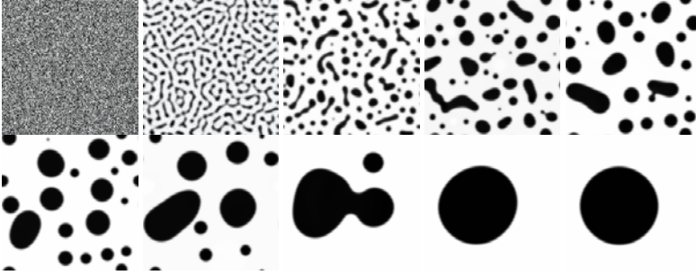
Figure 46. Time series of liquid-vapor phase separation dynamics in a 200 \times 200 \text{ lu}^2 domain. Gray scale proportional to normalized density. G = -120 , \psi_0 = 4 , \rho_0 = 200 , and \tau = 1 . Initial density 200 \text{ mu lu}^{-2} plus a random number in the interval [0,1] . Results shown at time = 0, 100, 200, 400, 800, 1600, 3200, 6400, 12800, and 25600 ts .
