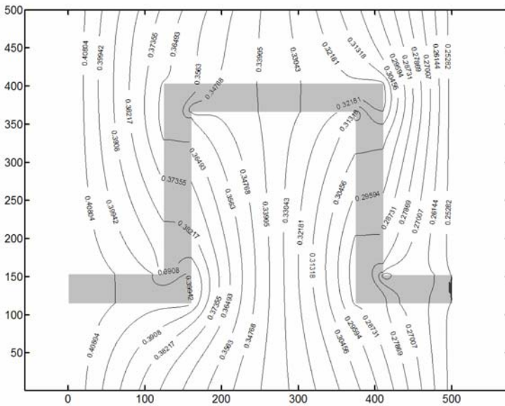
Figure 81. Pressure field in fractured porous medium analog. Porosity set to 0.8 to accentuate behavior of porous medium. \tau = 0.54 . The conduit (gray) plays an important role in determining the pressure field but there are significant gradients across the porous domain.
