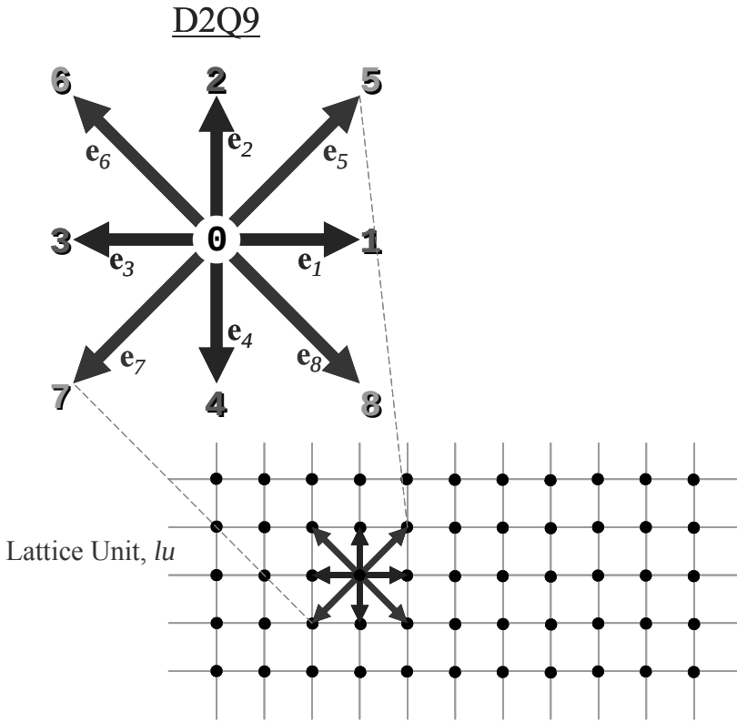
Figure 21. D2Q9 lattice and velocities.
