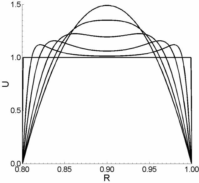
Figure 33. Simulated entry length effects in a slit using incompressible LBM. Velocity profiles at dimensionless distance from inlet Z = 0, 0.016, 0.033, 0.066, 0.1083 , and 0.245 (scaled relative to slit width of 0.2 ). Re = 100 . U is dimensionless velocity and R is dimensionless position relative to slit width of 0.2 . Compare with Figure 34.
