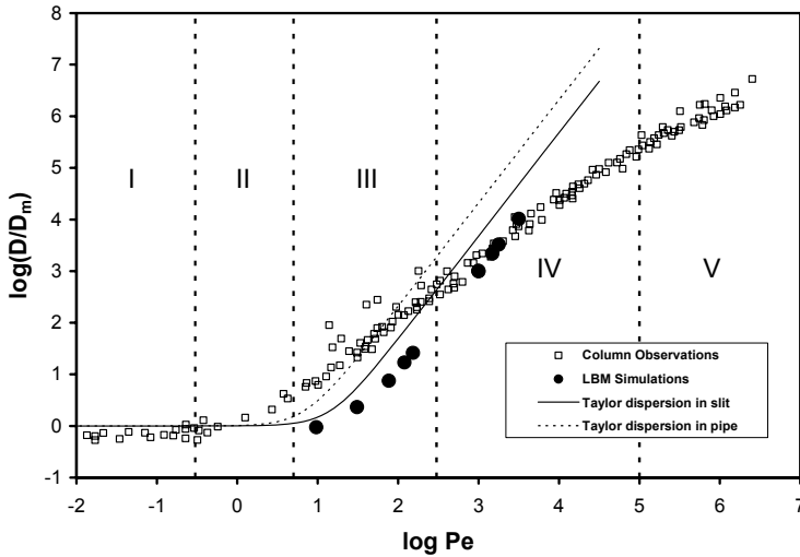
Figure 75. Empirical correlation between Péclet number and dimensionless dispersion coefficient (Modified from Fried and Combarnous, 1971, with permission). Regions I through V represent ranges of different behavior resulting from increasing relative importance of mechanical dispersion over diffusion. Observations mostly from packed columns, the results of LBM simulations as described below, and the Taylor-Aris theory predictions for slits and pipes are shown.
