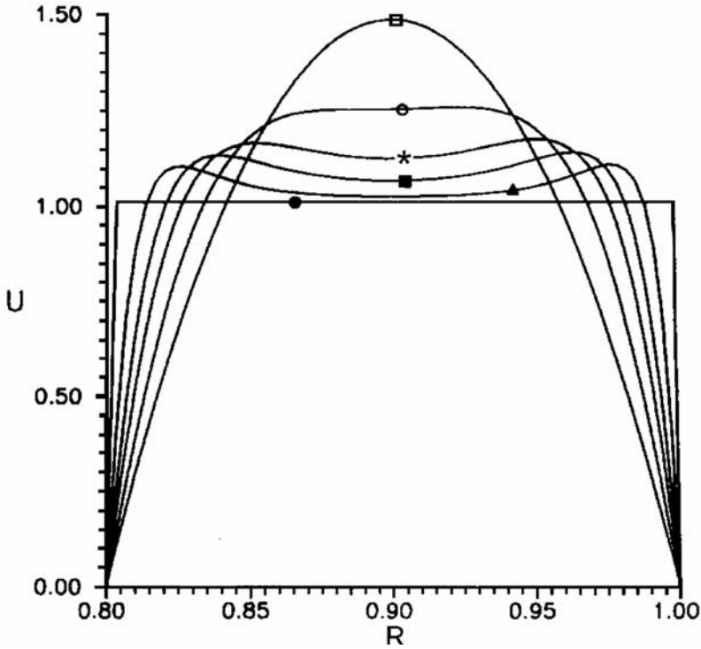
Figure 34. Entry length effects in annular space between two pipes. Velocity profiles at dimensionless distance from inlet Z = 0, 0.016, 0.033, 0.066, 0.1083 , and 0.245 (scaled relative to radius of large pipe). Re = 100 . U is dimensionless velocity and R is dimensionless radial position relative to radius of large pipe. (Reprinted from Nouar et al. (1995), Copyright (1995), with permission from Elsevier).
