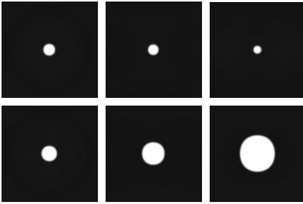
Figure 50. Effect of initial seed bubble size on evolution for \Delta P = -1 \mu\text{t s}^{-2} . Top: r = 12 \text{ lu} bubble dissipates due to condensation. Bottom: r = 15 \text{ lu} bubble nucleates cavitation.
